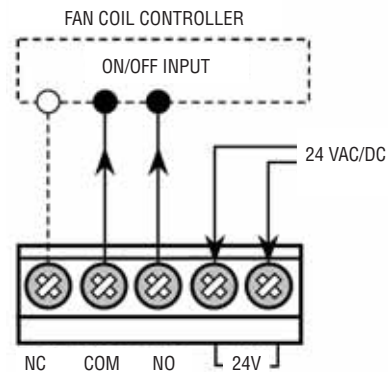
Figure 3 Wiring the Sensor
