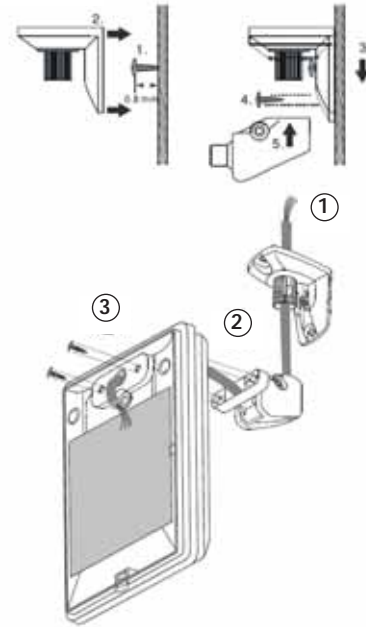
Figure 2 Mounting the Sensor
